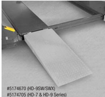
#5174670 (HD-9SW/SWX) #5174705 (HD-7 & HD-9 Series) Extended Alum. Approach Ramps Width - 19.75" / Length - 48"
