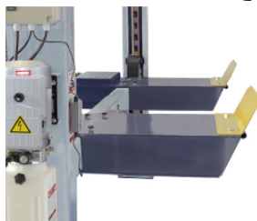
Optional platform extension kits add 660mm length to the runways.
