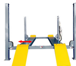
Adjustable runway: The off-side runway can be installed with a narrower or wider positioning.
